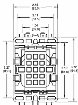
3 Pole Contactor 50 - 60 FLA
